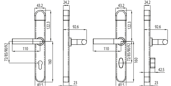
Int. Escutcheon with mech. cylinder and Openow (L3V)
